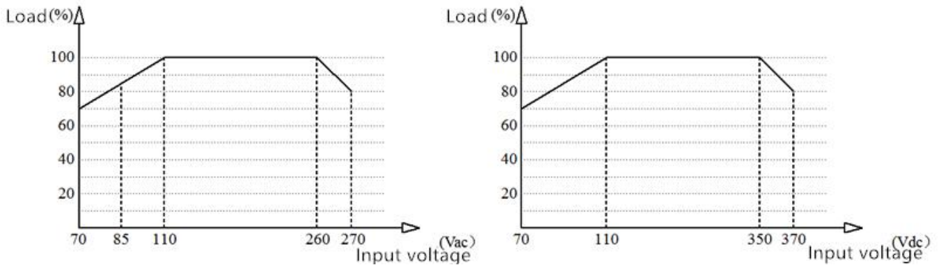
Input voltage and load characteristics curve
