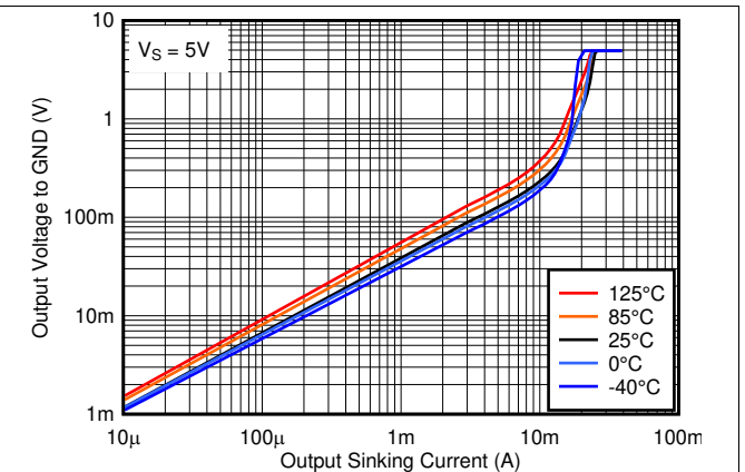
Figure 25. Output Low Voltage vs. Output Sinking Current at 5V
