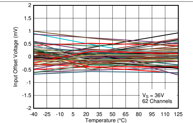
Figure 15. Input Offset Voltage vs. Temperature at 36V
