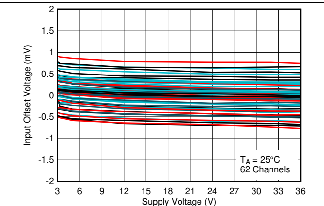
Figure 17. Input Offset Voltage vs. Supply Voltage at 25^\circ\text{C}
