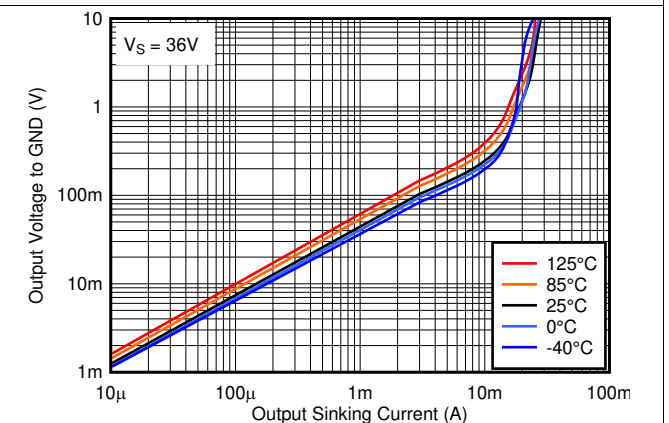
Figure 27. Output Low Voltage vs. Output Sinking Current at 36V
