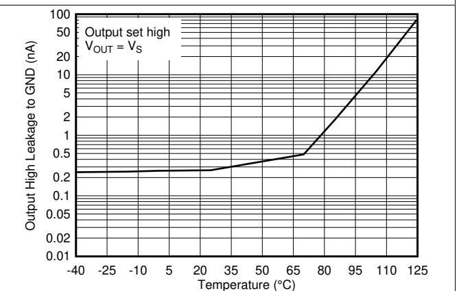
Figure 29. Output High Leakage Current vs. Temperature at 36V
