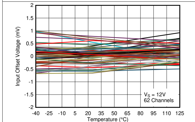
Figure 14. Input Offset Voltage vs. Temperature at 12V
