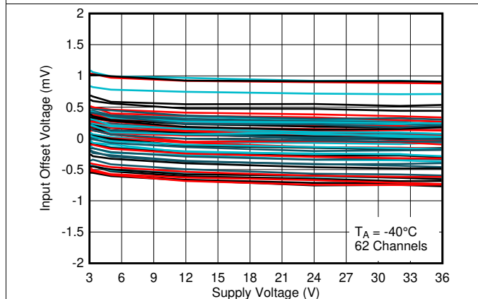
Figure 16. Input Offset Voltage vs. Supply Voltage at -40^\circ\text{C}
