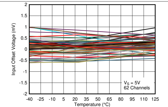
Figure 13. Input Offset Voltage vs. Temperature at 5V
