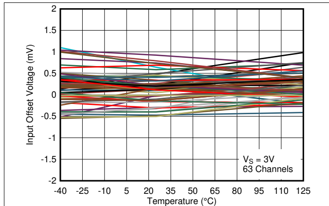
Figure 12. Input Offset Voltage vs. Temperature at 3V
