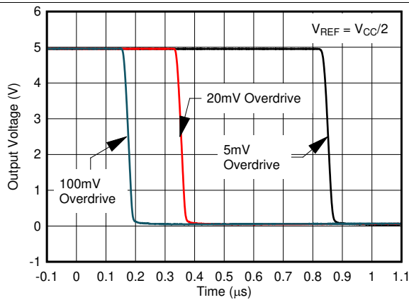
Figure 36. Response Time for Various Overdrives, High-to-Low Transition
