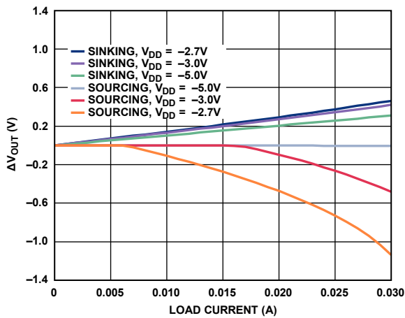
Figure 20. Headroom/Footroom ( \Delta V_{OUT} ) vs. Load Current
