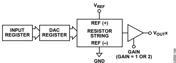
Figure 40. Single DAC Channel Architecture Block Diagram
