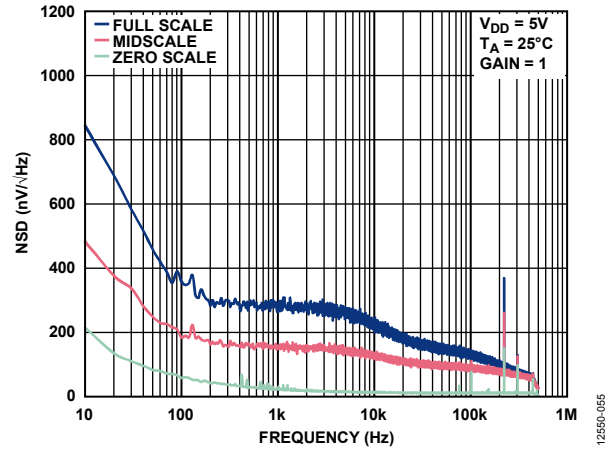
Figure 34. Noise Spectral Density (NSD)
