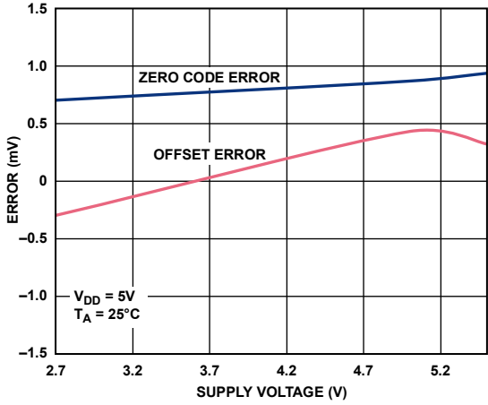
Figure 18. Zero Code Error and Offset Error vs. Supply Voltage
