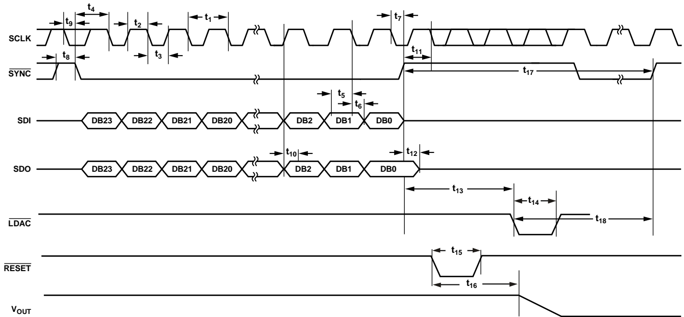
Figure 4. SPI Timing Diagram, Compatible with Mode 1 and Mode 2 (See the AN-1248 Application Note)
