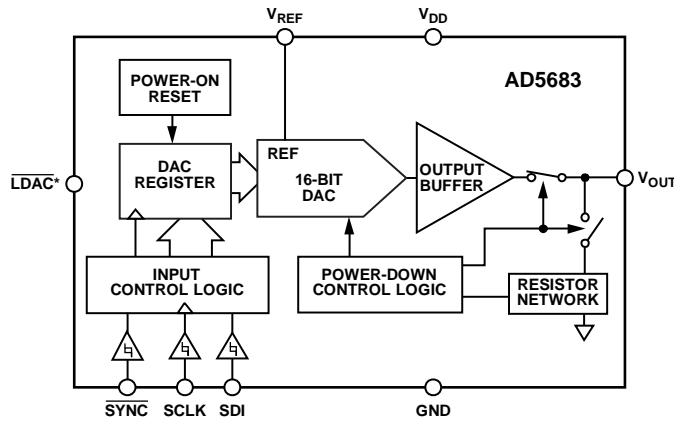
Figure 3. AD5683 LFCSP
