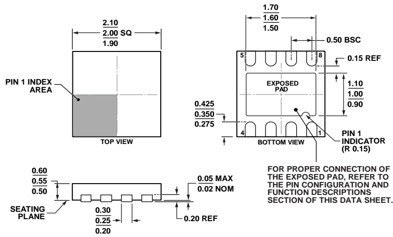
Figure 56. 8-Lead Lead Frame Chip Scale Package [LFCSF_UD] 2.00 mm × 2.00 mm Body, Ultra Thin, Dual Lead (CP-8-10)
