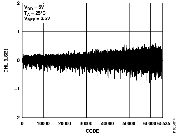
Figure 14. AD5683R/AD5683 DNL
