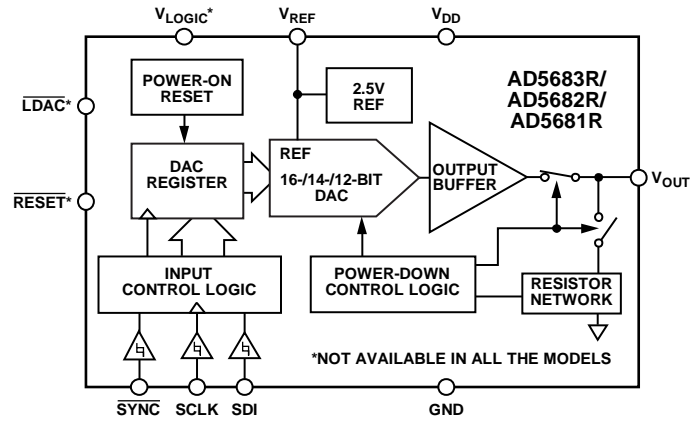
Figure 2. AD5683R/AD5682R/AD5681R LFCSP
