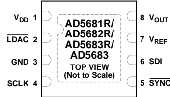
Figure 6. Pin Configuration, 8-Lead LFCSP, \overline{\text{LDAC}} Option
