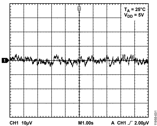
Figure 31. 0.1 Hz to 10 Hz Output Noise Plot, Internal Reference On
