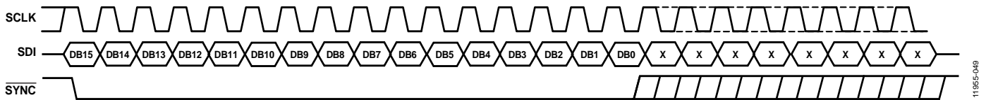
Figure 49. Short Write on the AD5681R
