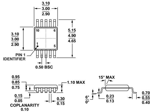
COMPLIANT TO JEDEC STANDARDS MO-187-BA Figure 57. 10-Lead Mini Small Outline Package [MSOP] (RM-10)
