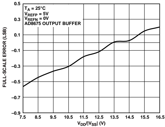
Figure 24. Full-Scale Error vs. Supply Voltage, 5 V Span
