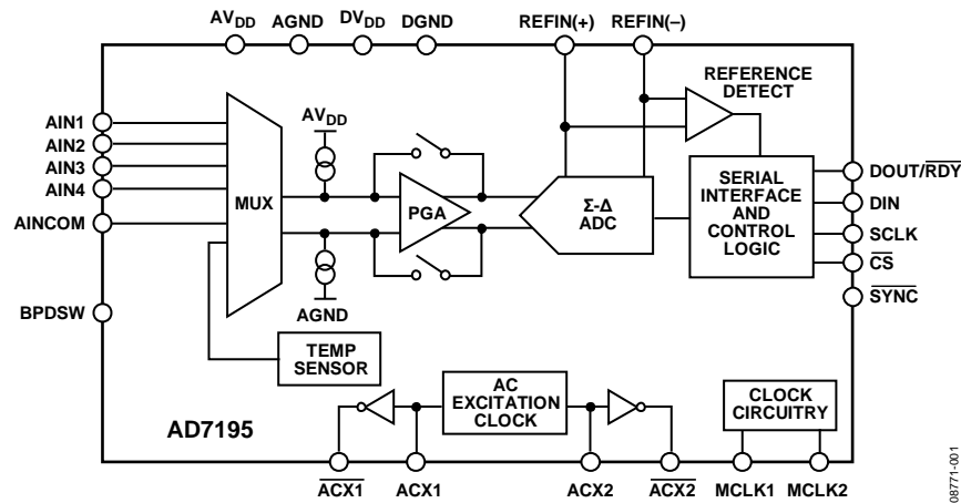
Figure 18. Block Diagram
