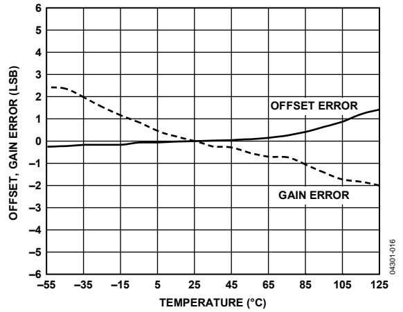
Figure 20. Offset and Gain Error vs. Temperature
