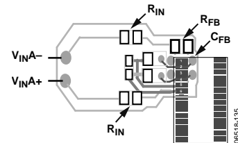
Figure 53. Typical Layout Structure for Surrounding Components
