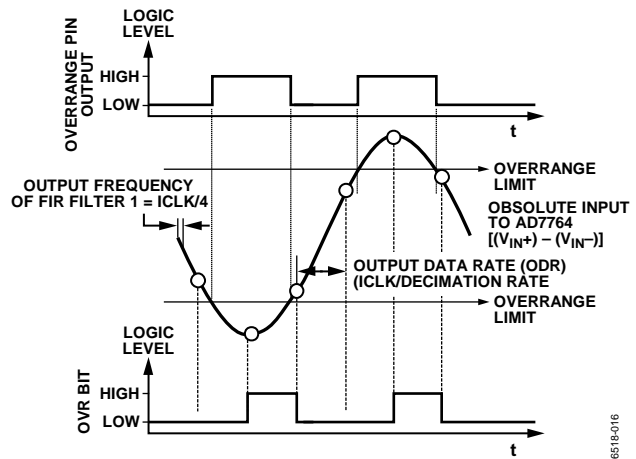
Figure 42. OVERRANGE Pin and OVR Bit vs. Absolute Voltage Applied to the Modulator
