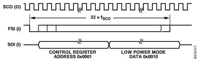
Figure 43. Write Scheme for Low Power Mode
