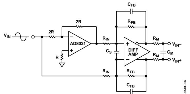
Figure 37. Single-Ended-to-Differential Conversion
