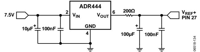
Figure 52. Reference Connection
