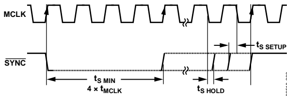
Figure 41. SYNC Timing Relative to MCLK
