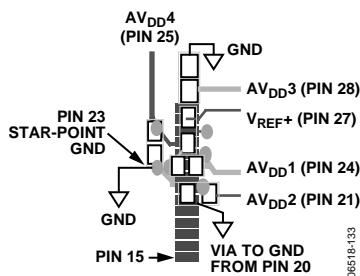
Figure 51. Supply Decoupling
