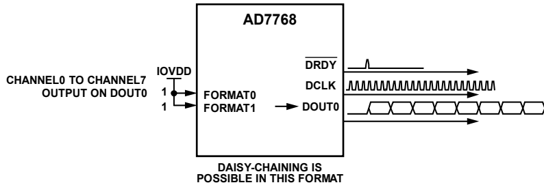
Figure 95. AD7768 FORMATx = 10 or 11, or AD7768-4 FORMAT0 = 1, One Data Output Pin
