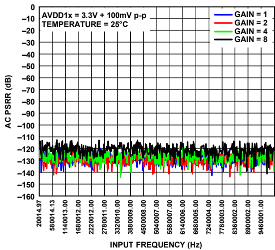
Figure 64. AC Power Supply Rejection Ratio (PSRR) vs. Input Frequency at 16 kSPS, High Resolution Mode
