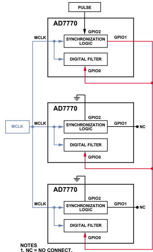
Figure 108. Hardware ODR Update
