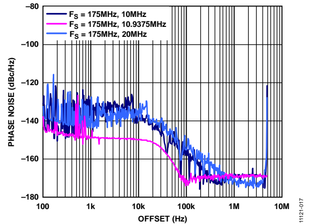
Figure 17. Phase Noise
