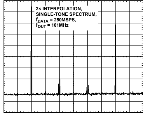
Figure 13. Single-Tone Spectrum, 2× Interpolation, f_{DATA} = 250 MSPS, f_{OUT} = 101 MHz
