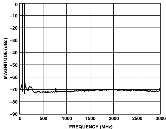
Figure 65. Eight Carriers at 70 MHz Output (Shuffle On)
