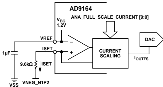
Figure 135. Voltage Reference Circuit
