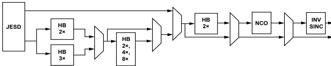
Figure 109. Block Diagram of the Main Digital Datapath
