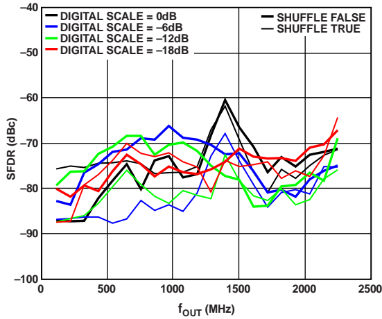
Figure 18. SFDR vs. f_{OUT} over Digital Scale
