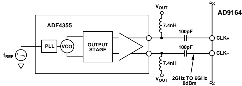
Figure 136. Possible Signal Chain for CLK± Input
