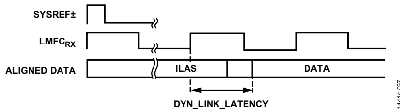
Figure 106. DYN_LINK_LATENCY_x Illustration
