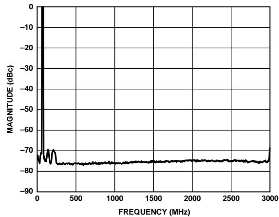
Figure 64. Four Carriers at 70 MHz Output (Shuffle On)
