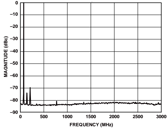
Figure 63. Single Carrier at 70 MHz Output (Shuffle On)
