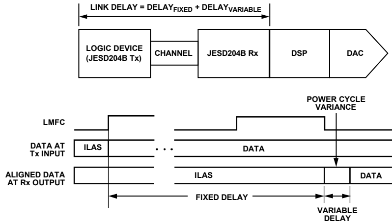
Figure 102. JESD204B Link Delay = Fixed Delay + Variable Delay
