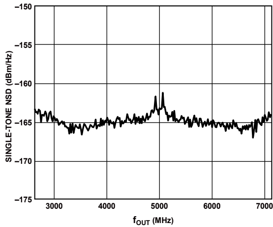
Figure 44. Single-Tone NSD vs. f_{OUT}
