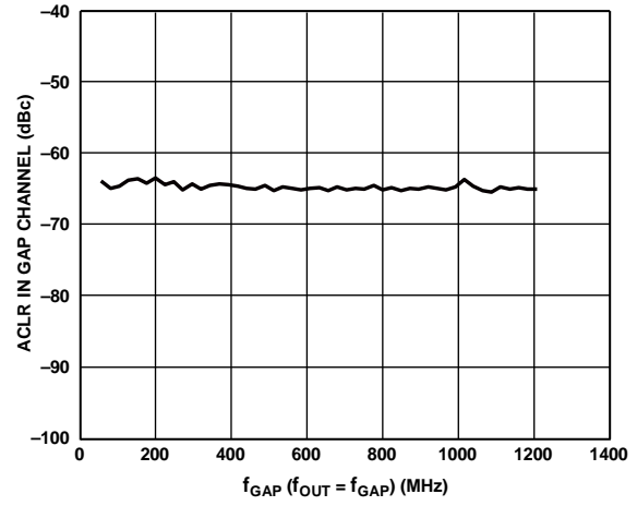
Figure 85. ACLR in Gap Channel vs. f_{GAP}
