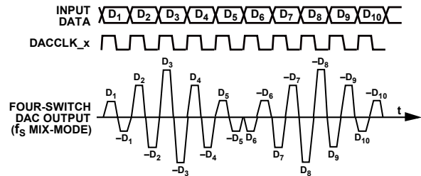
Figure 130. Mix-Mode Waveform
