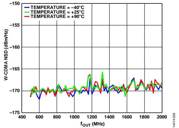
Figure 33. W-CDMA NSD Measured at 70 MHz vs. f_{OUT} over Temperature
