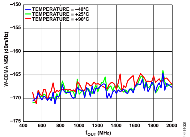
Figure 34. W-CDMA NSD Measured at 10% Offset from f_{OUT} vs. f_{OUT} over Temperature
