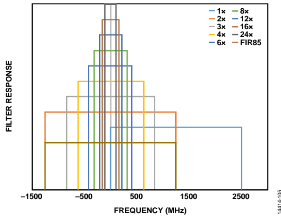
Figure 110. All Band Responses of Interpolation Filters
