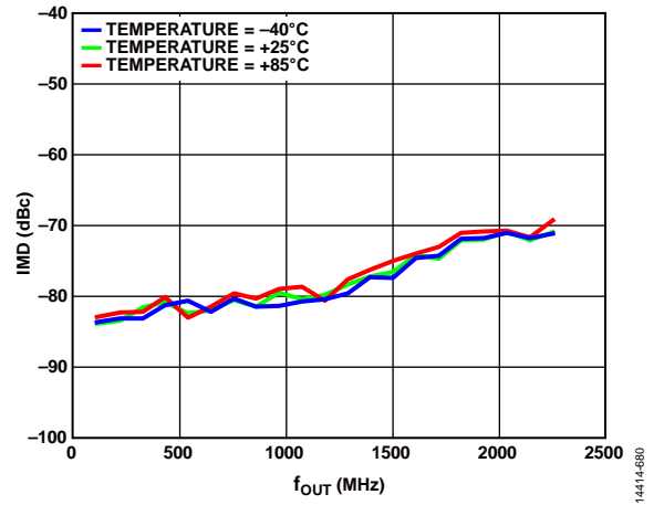
Figure 29. IMD vs. f_{OUT} over Temperature
