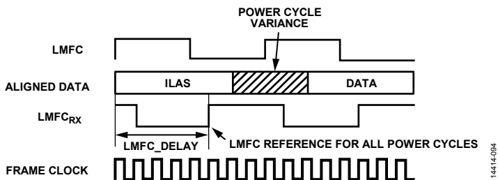
Figure 104. LMFC_DELAY_x to Compensate for Link Delay > LMFC
