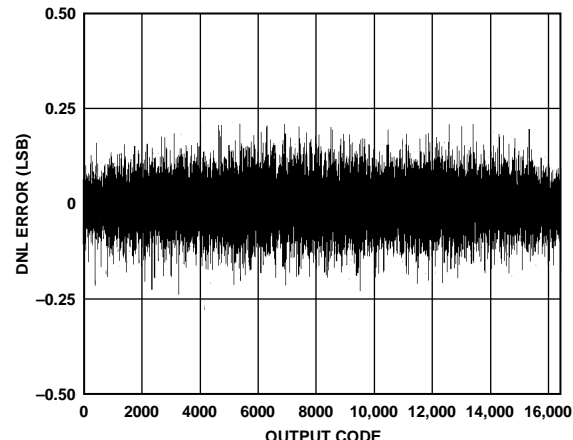
Figure 29. AD9255-105 DNL with f_{IN} = 12.5 MHz
