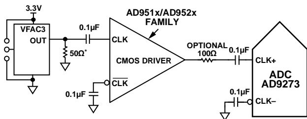
Figure 58. Single-Ended 1.8 V CMOS Sample Clock
