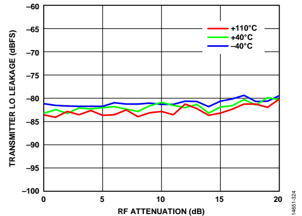
Figure 24. Transmitter LO Leakage vs. RF Attenuation, 900 MHz LO, Transmitter QEC and External LO Leakage Tracking Active, CW Signal 5 MHz Offset from LO, 6 dB Digital Backoff, 1 MHz Measurement Bandwidth (If Input Power to ORx Channel Is Not Held Constant, Performance Degrades As Shown in This Plot)
