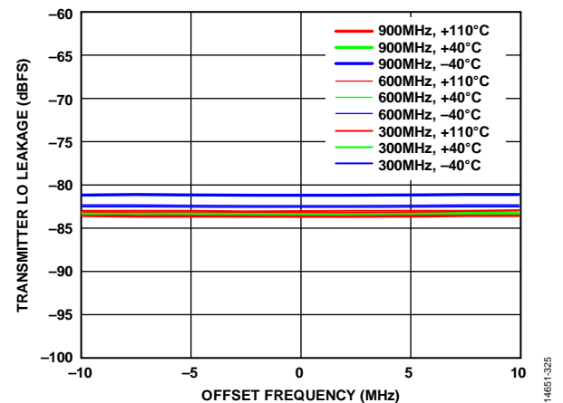
Figure 25. Transmitter LO Leakage vs. Offset Frequency, Transmitter QEC and External LO Leakage Tracking Active, 5 dB Digital Backoff, 1 MHz Measurement Bandwidth
