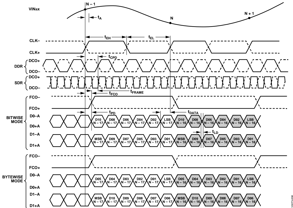
Figure 4. 12-Bit DDR/SDR, Two-Lane, 2x Frame Mode
