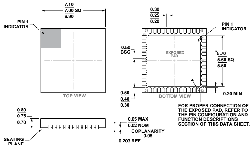
Figure 76. 48-Lead Lead Frame Chip Scale Package [LFCSP_WQ] 7 mm × 7 mm Body, Very Very Thin Quad (CP-48-13) Dimensions shown in millimeters
