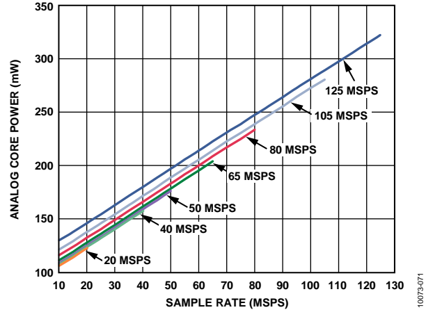
Figure 68. Analog Core Power vs. f_{SAMPLE} for f_{IN} = 10.3 \text{ MHz}
