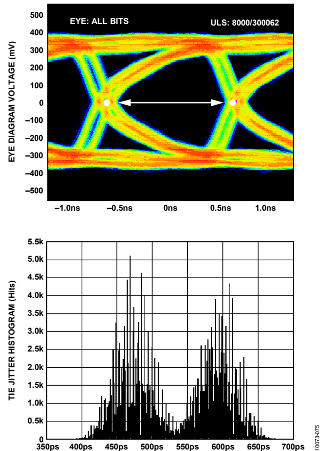
Figure 71. Data Eye for LVDS Outputs in ANSI-644 Mode with Trace Lengths Less than 24 Inches on Standard FR-4 Material, External 100 Ω Far-End Termination Only
