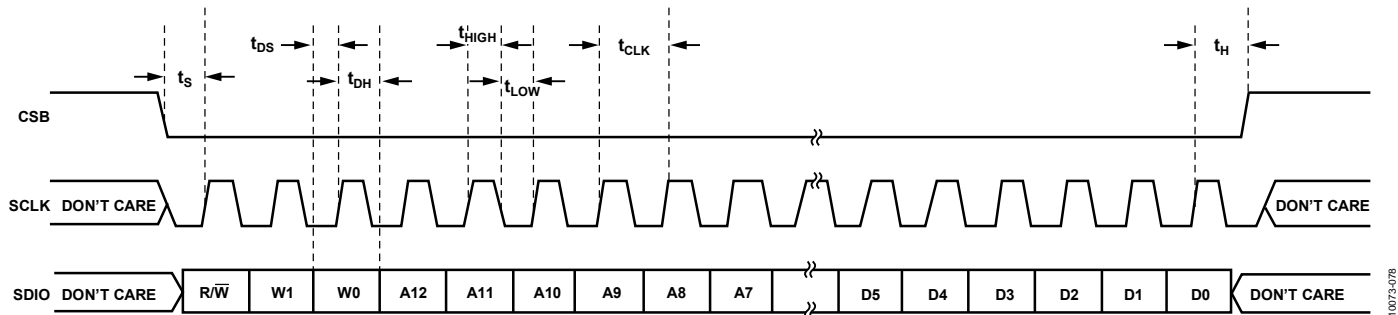
Figure 73. Serial Port Interface Timing Diagram
