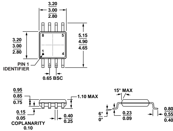
COMPLIANT TO JEDEC STANDARDS MO-187-AA Figure 89. 8-Lead Mini Small Outline Package [MSOP] (RM-8) Dimensions shown in millimeters
