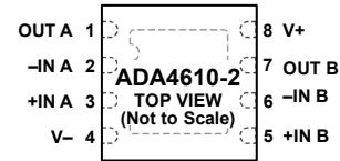
Figure 6. ADA4610-2 Pin Configuration, 8-Lead LFCSP (CP Suffix)
