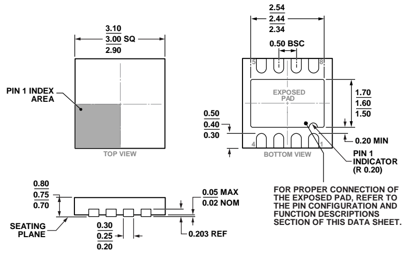
Figure 64. 8-Lead Lead Frame Chip Scale Package [LFCSP] 3 mm x 3 mm Body and 0.75 mm Package Height (CP-8-21) Dimensions shown in millimeters
