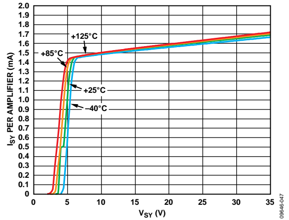
Figure 52. Supply Current ( I_{SV} ) per Amplifier vs. Supply Voltage ( V_{SY} ) at Various Temperatures
