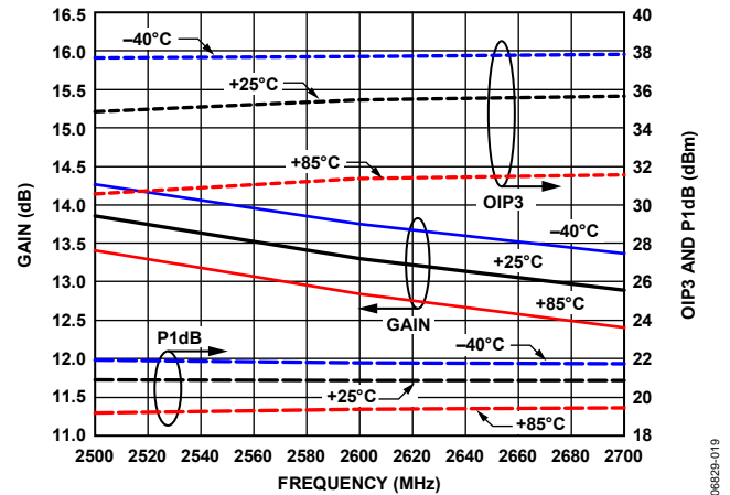
Figure 19. Gain, OIP3, and P1dB vs. Temperature
