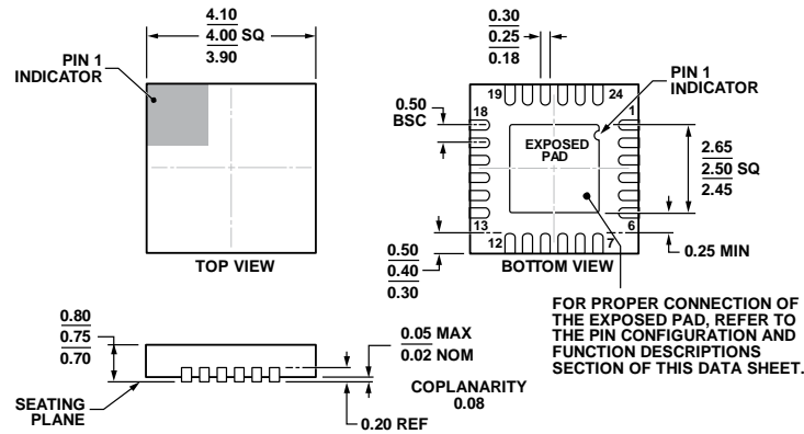
Figure 40. 24-Lead Lead Frame Chip Scale Package [LFCSP_WQ] 4 mm × 4 mm Body, Very Very Thin Quad (CP-24-7) Dimensions shown in millimeters
