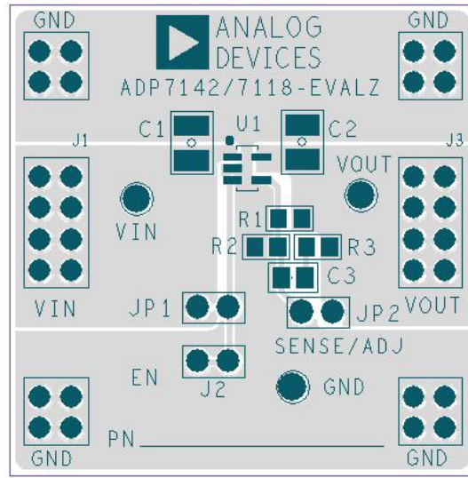
Figure 66. Example TSOT PCB Layout
