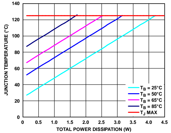
Figure 61. LFCSP Junction Temperature Rise, Different Board Temperatures
