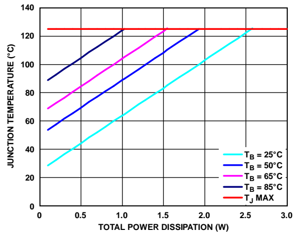
Figure 62. SOIC Junction Temperature Rise, Different Board Temperatures
