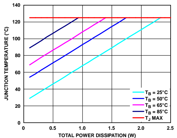
Figure 63. TSOT Junction Temperature Rise, Different Board Temperatures
