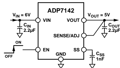
Figure 1. ADP7142 with Fixed Output Voltage, 5 V
