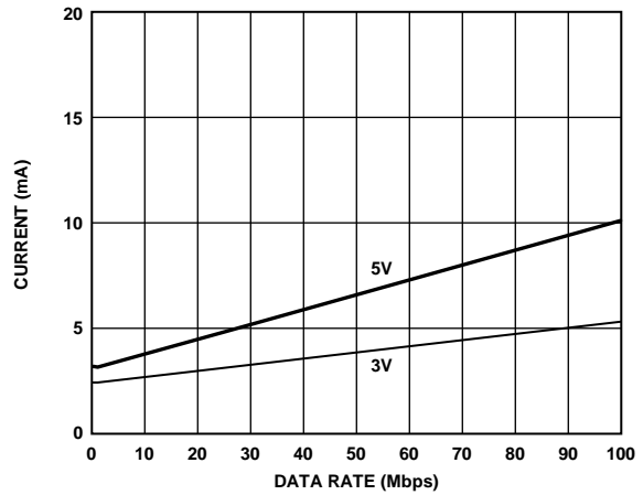
Figure 10. Typical ADuM1280 or ADuM1285 V_{DD2} Supply Current vs. Data Rate for 5 V and 3 V Operation
