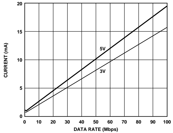
Figure 9. Typical ADuM1280 or ADuM1285 V_{DD1} Supply Current vs. Data Rate for 5 V and 3 V Operation
