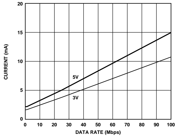
Figure 11. Typical ADuM1281 or ADuM1286 V_{DD1} or V_{DD2} Supply Current vs. Data Rate for 5 V and 3 V Operation
