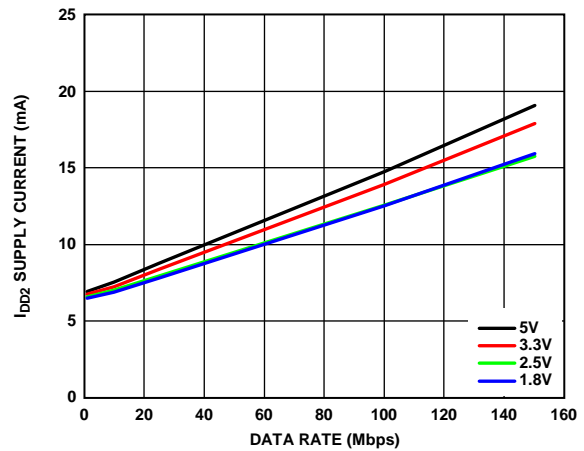
Figure 15. ADuM162N I_{DD2} Supply Current vs. Data Rate at Various Voltages
