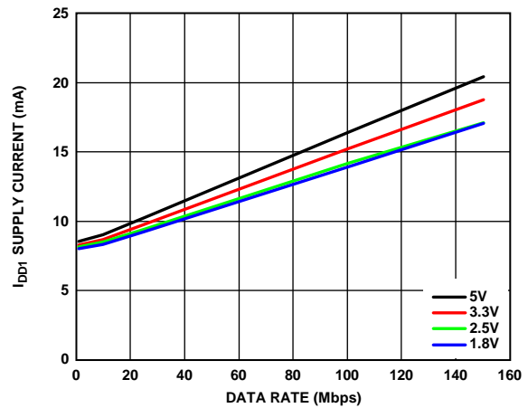
Figure 14. ADuM162N I_{DD1} Supply Current vs. Data Rate at Various Voltages
