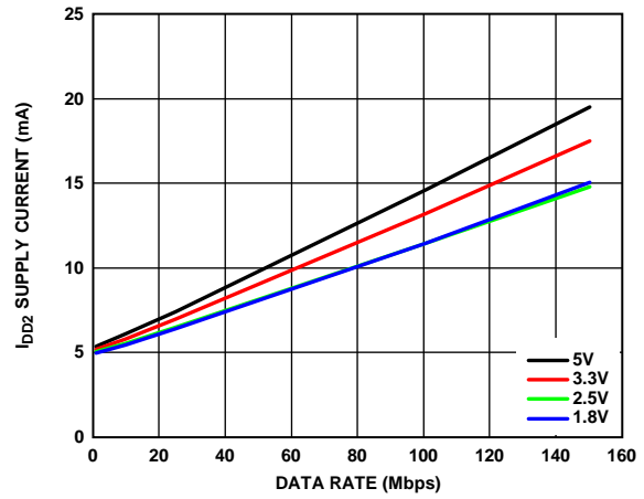
Figure 13. ADuM161N I_{DD2} Supply Current vs. Data Rate at Various Voltages
