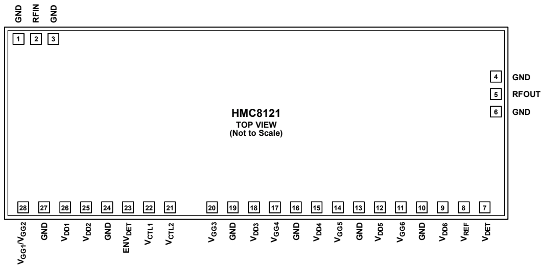
Figure 2. Pad Configuration
