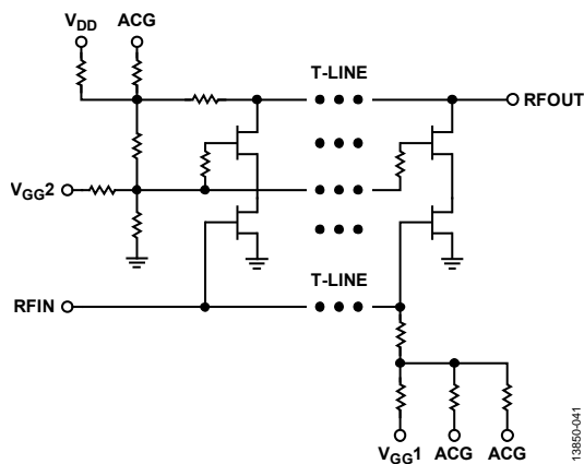
Figure 41. Architecture and Simplified Schematic
