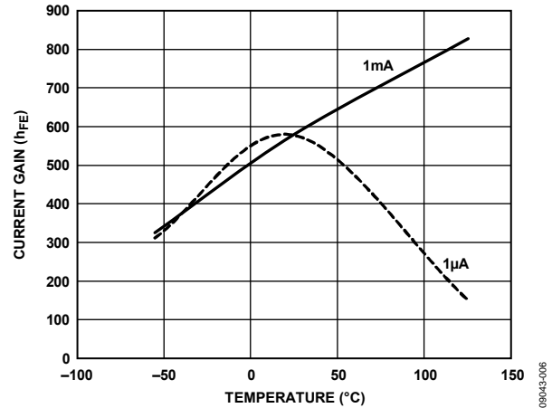
Figure 7. Current Gain vs. Temperature (Excludes I CB0 )
