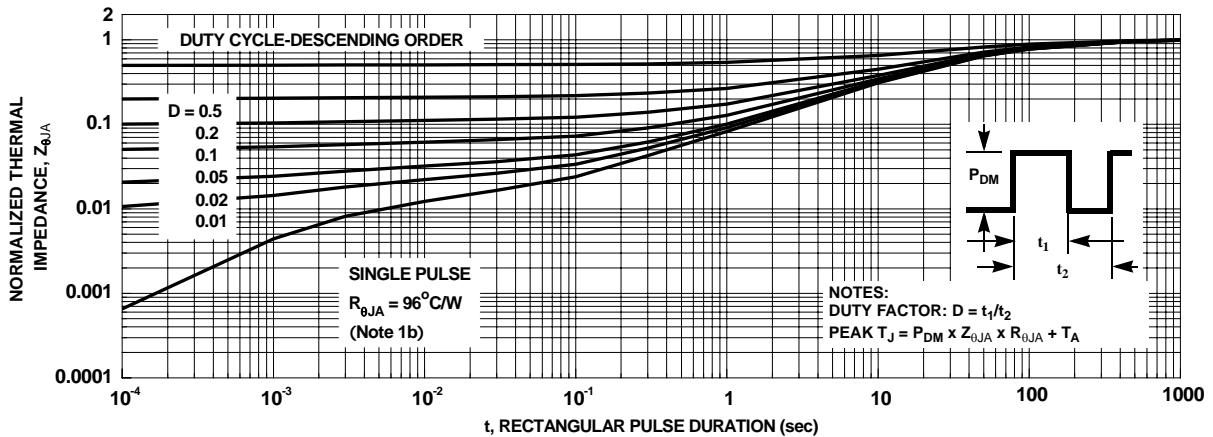
Figure 15. Transient Thermal Response Curve
