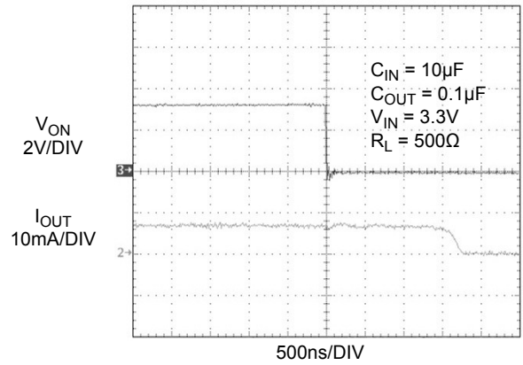
Figure 16. t_{dOFF} Response
