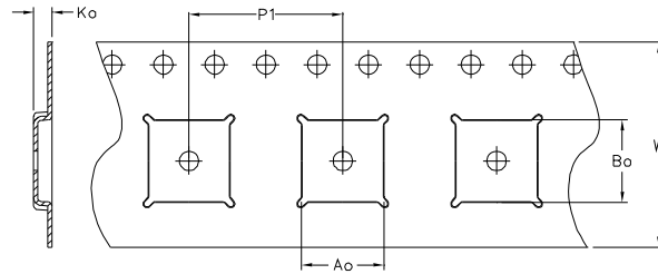
TAPE DIMENSIONS
