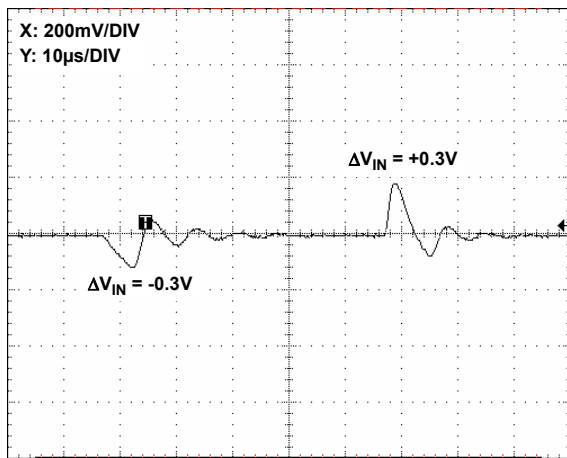
FIGURE 23. LINE TRANSIENT RESPONSE, 0.001 \mu F LOAD CAPACITANCE
