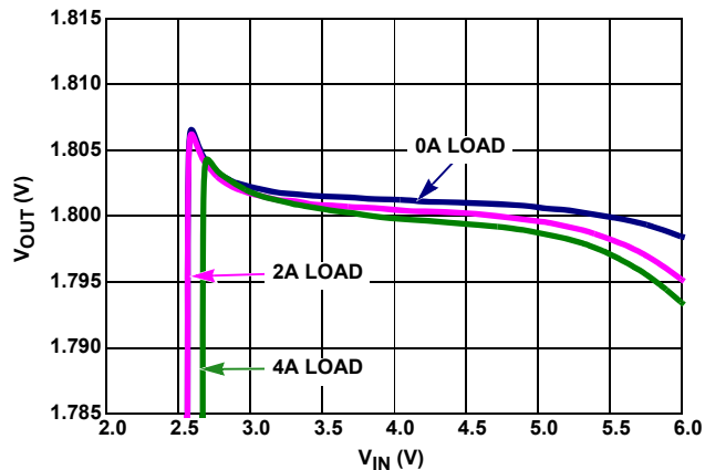
FIGURE 14. OUTPUT VOLTAGE REGULATION vs V_{IN} (PWM V_{OUT} = 1.8\text{V} )
