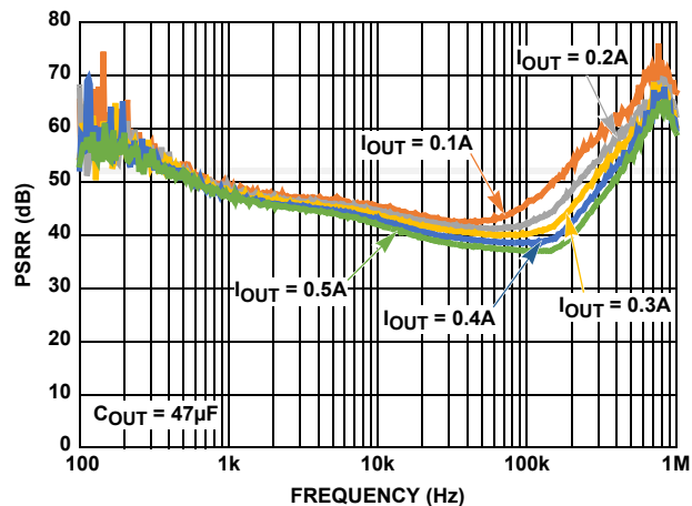
FIGURE 27. PSRR vs FREQUENCY ( C_{\text{OUT}} = 47\mu\text{F} )
