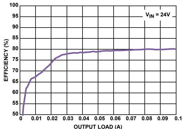
FIGURE 24. EFFICIENCY vs LOAD, PFM, V_{OUT} = 3.3V
