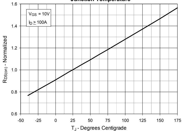
Fig. 4. Normalized R_{DS(on)} to I_D = 100A Value vs. Junction Temperature
