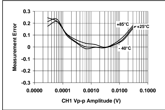
FIGURE 2-19: Measurement Error w/ External V_{REF} ( G = 16 ).
