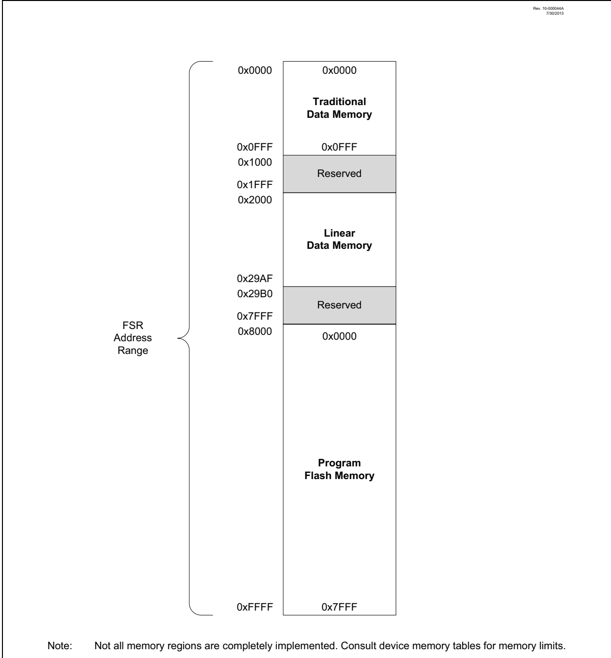
FIGURE 3-9: INDIRECT ADDRESSING
