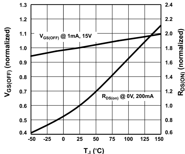
V GS(OFF) and R DS(ON) w/ Temperature
