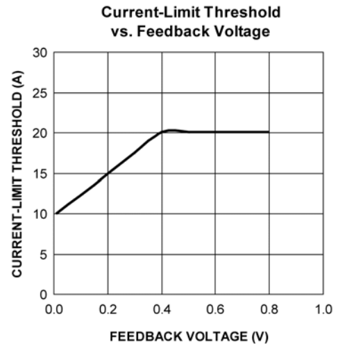
Figure 5. MIC24056 Current-Limit Foldback Characteristic
