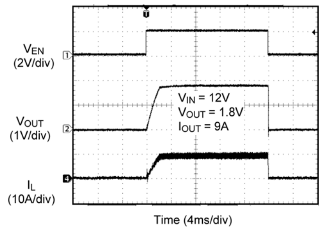
Enable Turn-On/Turn-Off
