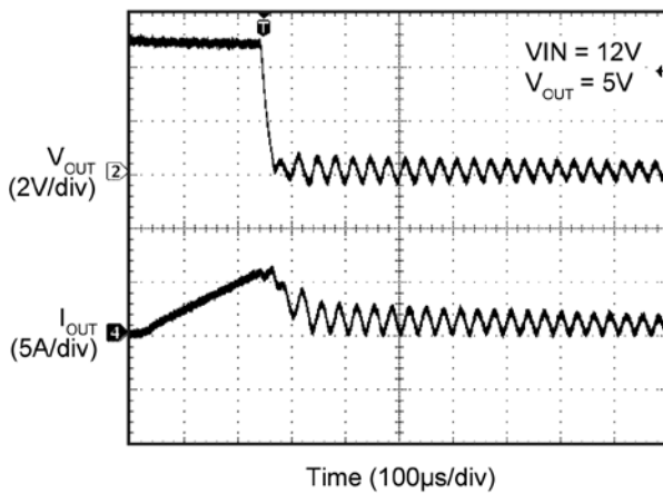
Short Circuit
