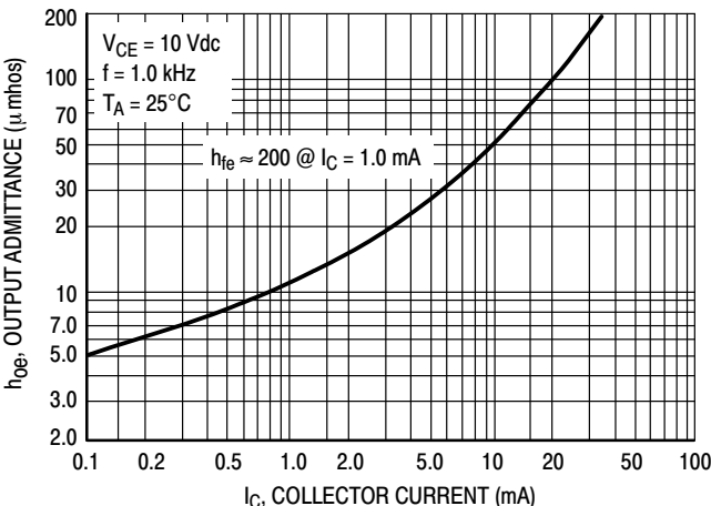
Figure 18. Output Admittance
