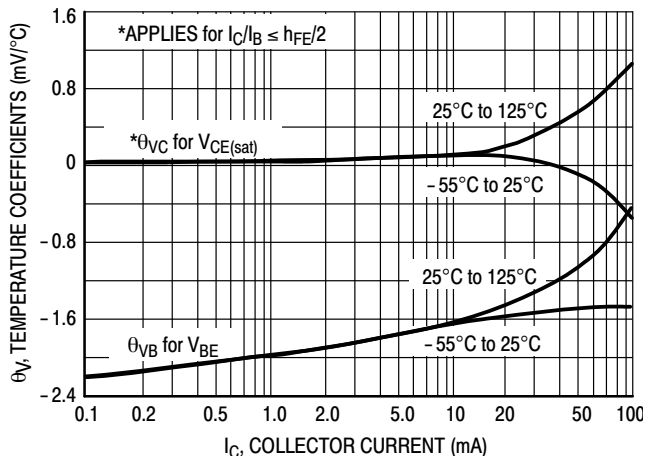
Figure 12. Temperature Coefficients
