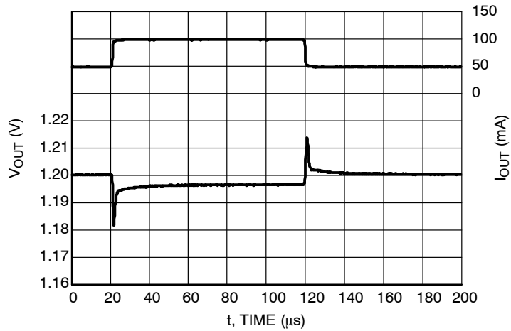
Figure 68. Load Transients, 1.2 V Version, I_{OUT} = 50 - 100 \text{ mA} , t_R = t_F = 0.5 \mu s , V_{IN} = 2.2 \text{ V} , AE = V_{IN} \text{ V}
