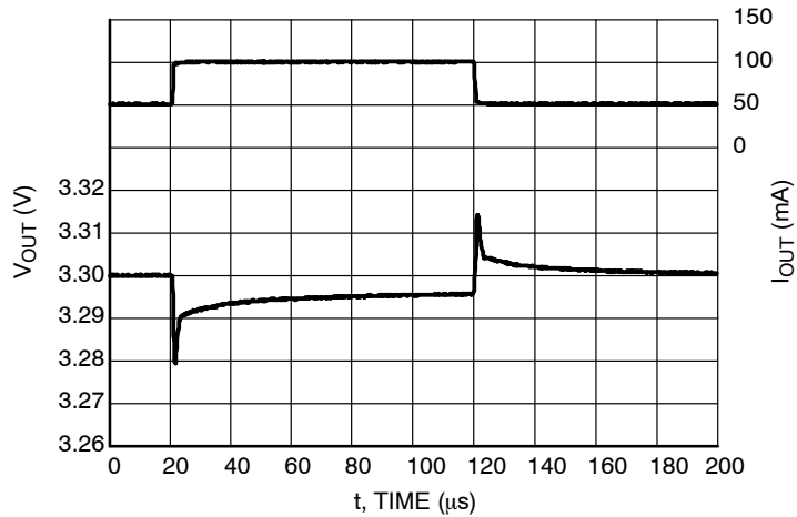
Figure 70. Load Transients, 3.3 V Version, I_{OUT} = 50 - 100 \text{ mA} , t_R = t_F = 0.5 \mu s , V_{IN} = 4.3 \text{ V} , AE = V_{IN} \text{ V}
