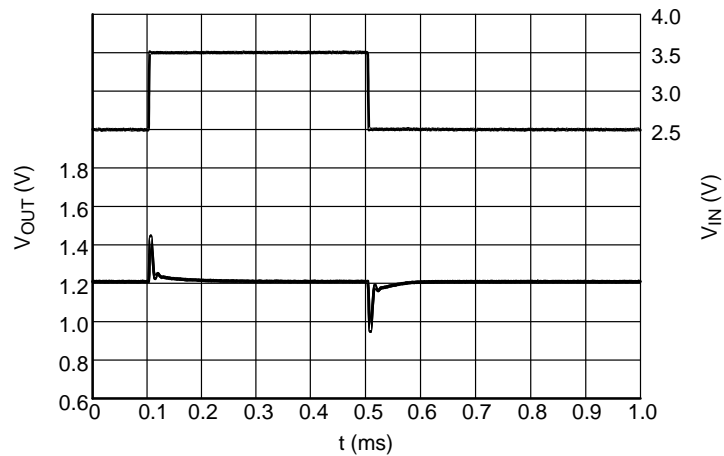
Figure 24. Line Transients, 1.2 V Version, I_{OUT} = 1 \text{ mA}
