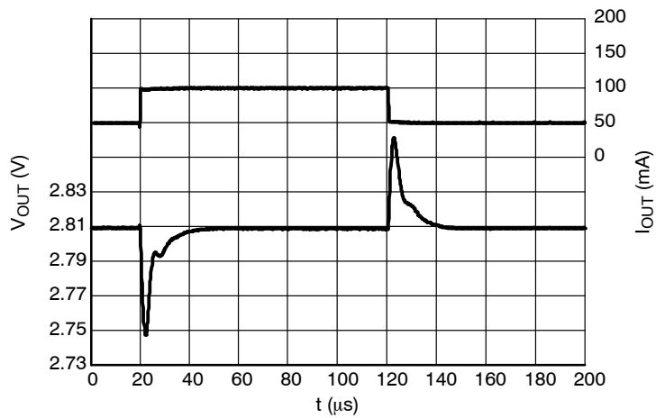
Figure 30. Load Transients, 2.8 V Version, I_{\text{OUT}} = 50 - 100 \text{ mA} , t_{\text{R}} = t_{\text{F}} = 0.5 \mu\text{s} , V_{\text{IN}} = 3.8 \text{ V}
