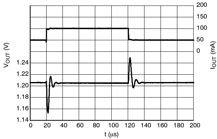
Figure 29. Load Transients, 1.2 V Version, I_{\text{OUT}} = 50 - 100 \text{ mA} , t_{\text{R}} = t_{\text{F}} = 0.5 \mu\text{s} , V_{\text{IN}} = 2.6 \text{ V}
