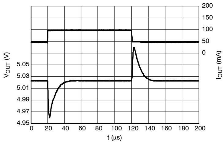
Figure 31. Load Transients, 5.0 V Version, I_{\text{OUT}} = 50 - 100 \text{ mA} , t_{\text{R}} = t_{\text{F}} = 0.5 \mu\text{s} , V_{\text{IN}} = 6.0 \text{ V}
