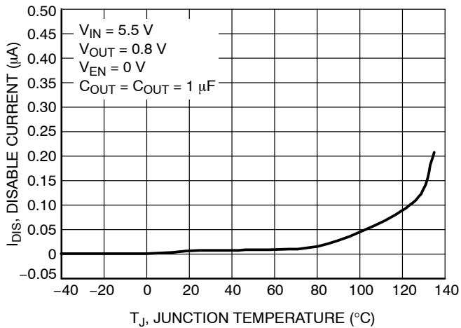
Figure 31. Disable Current vs. Temperature, V_{OUT} = 0.8\text{ V}
