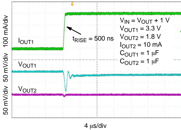
Figure 42. Load Transient Response – 3.3 V – Rising Edge, IOUT1 = 100 μA to 300 mA
