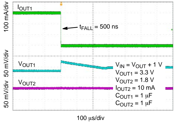
Figure 43. Load Transient Response – 3.3 V – Falling Edge, IOUT1 = 300 mA to 100 μA
