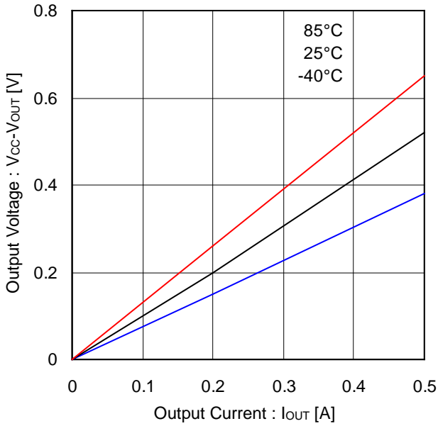
Figure 25. Output Voltage vs Output Current (Output High Voltage, BD6230)
