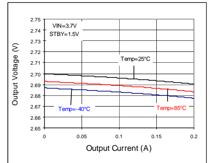
Fig 160. Load Regulation
