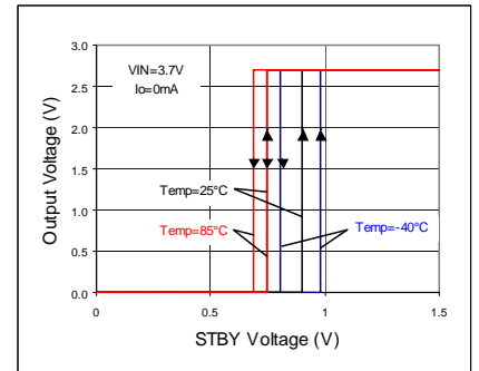
Fig 163. STBY Threshold
