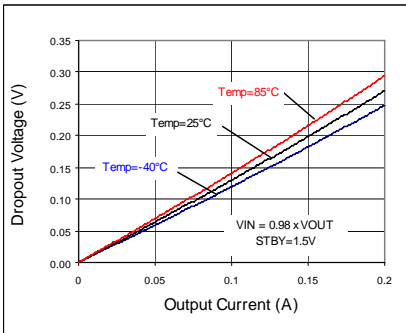
Fig 161. Dropout Voltage
