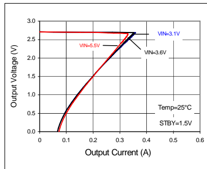
Fig 162. OCP Threshold
