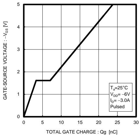
Fig.13 Dynamic Input Characteristics
